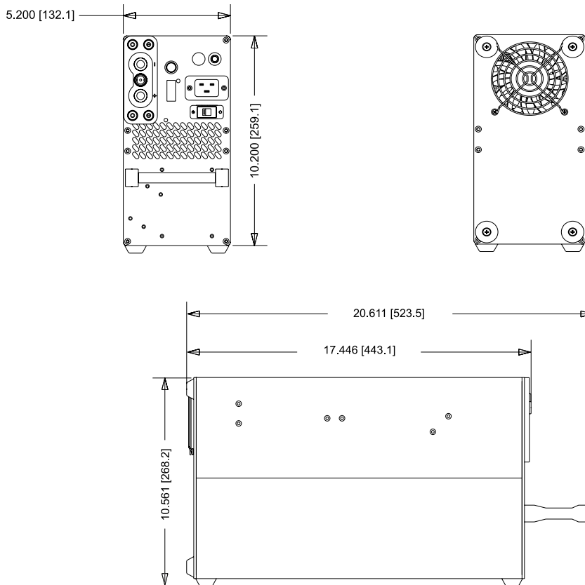
Figure 2.5.1 – TI1000 GPU-24 physical dimensions
