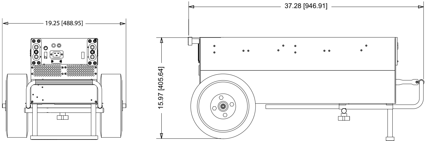
Figure 2.5.1 – TI2560 12-24 GPU physical dimensions
