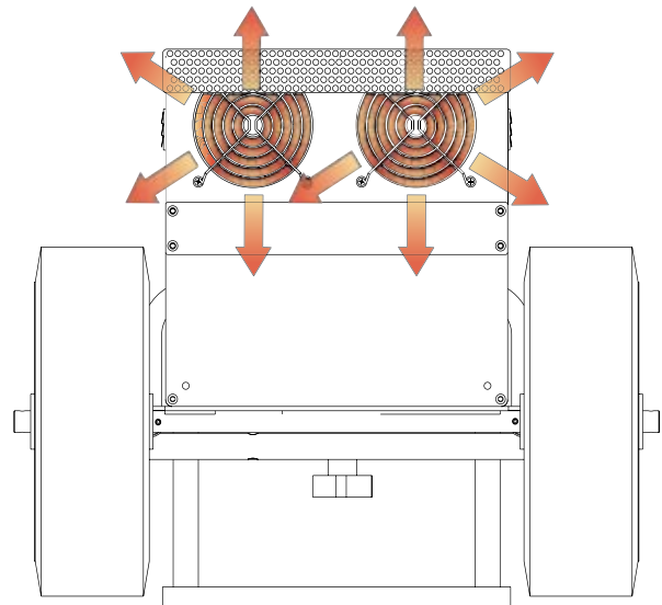
Figure 2.7.4: Rear Outlet
